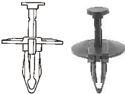
14019 (Ford: N803421-S; Chry: 6501590) Black Nylon Push-Type Retainer Head Dia: 1" Shoulder Length: 1/8" Stem Length: 7/8" Fits Into 5/16" Hole UNIT PACKAGE: 25
