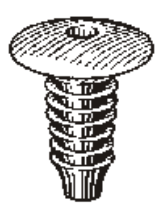
16132 Black Nylon Trim Panel Retainer Head Dia: 19mm Stem Length: 20mm Fits Into 8mm Hole UNIT PACKAGE: 25
