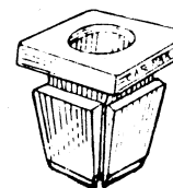
80-5236 Replaces: 26023-H1000 NUT-HEADLAMP ADJUSTING Hole: M8sq., Screw: M4.8 Nissan UNIT PACKAGE 25
