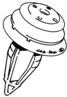
99-8342 Replaces: 01553-09791 RETAINER - DOOR PANEL Plastic Hole: M8, Upper Hd.: 13MM, Trim Thk: 2.5MM, O/L: 20MM, P.R.: 1.5MM Nissan 2000/ & Infinity '99/ UNIT PACKAGE 15
