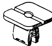
83-5690 Replaces: 68425-H5000, 9991-00-503,90662-671-0030 NUT Hole: M8sq., Screw: M4.2 Nissan, Mazda, Honda & General Usage UNIT PACKAGE 25
