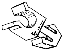
95-7466 Replaces: 53452-90351 CLIP-HOOD ROD PROP 6mm x 7mm Rod Dia.: Toyota Car & Truck '91/ UNIT PACKAGE 5
